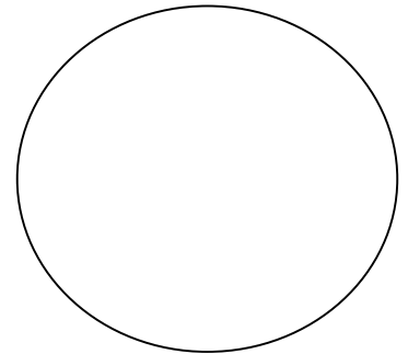
Adaptation 3
