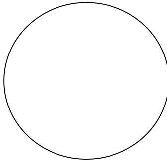
Adaptation 2
