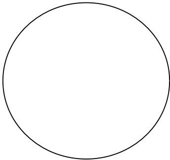
Adaptation 1
